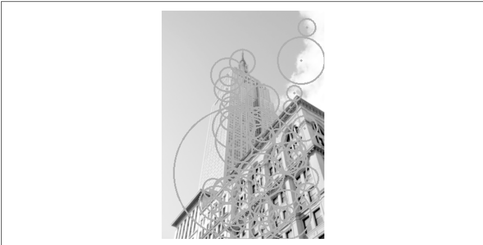
Figure 10-3. Sample SURF features extracted and plotted using OpenCV.
