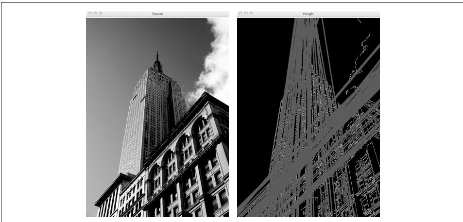
Figure 10-10. An example of detecting lines using a Hough transform. The left image is the source in grayscale. The right image shows an edge map with detected lines.
